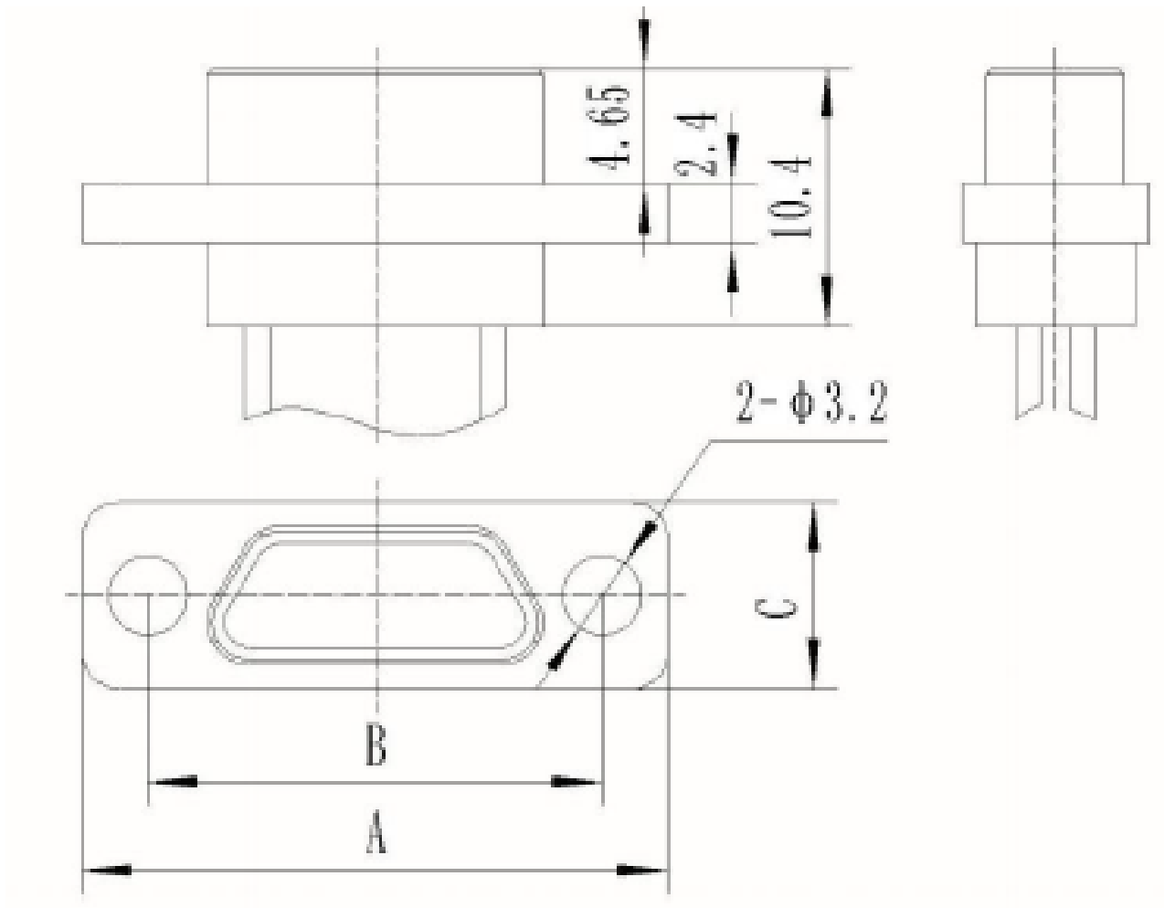
Figure D1: Outline & Dimensions
