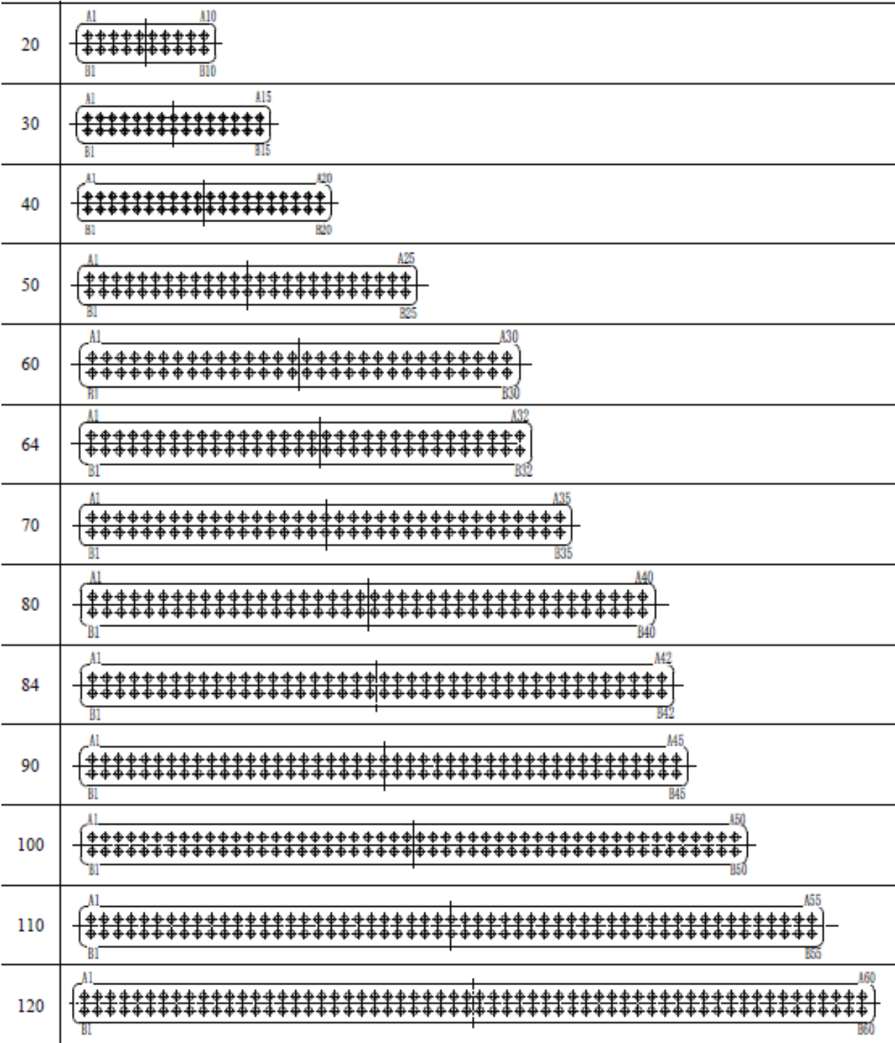
Figure D1: Outline & Dimensions
